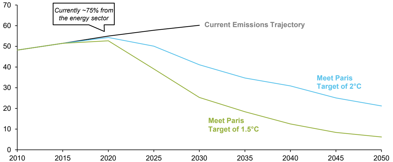
Source: UNEP Emission Gap Report 2019, IEA
